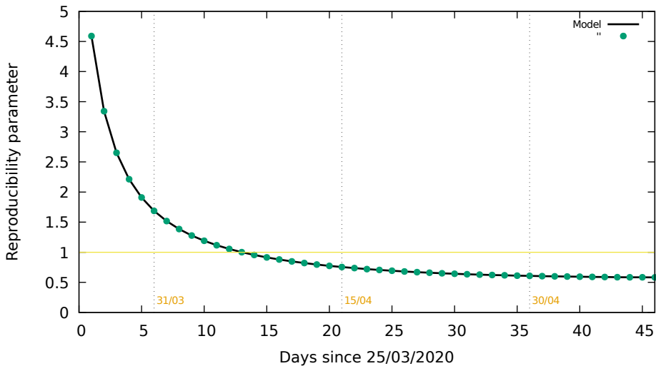
Murcia region, only PCR
