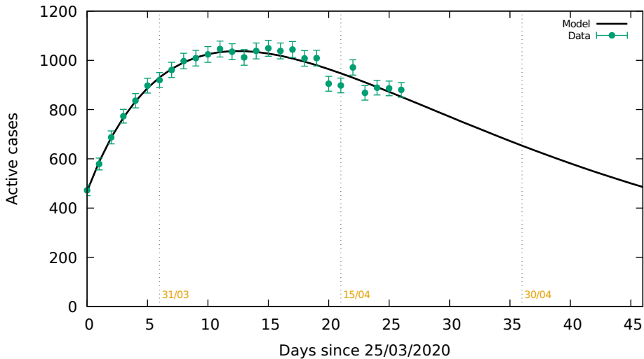
Murcia region, only PCR. Date 20/04/2020
