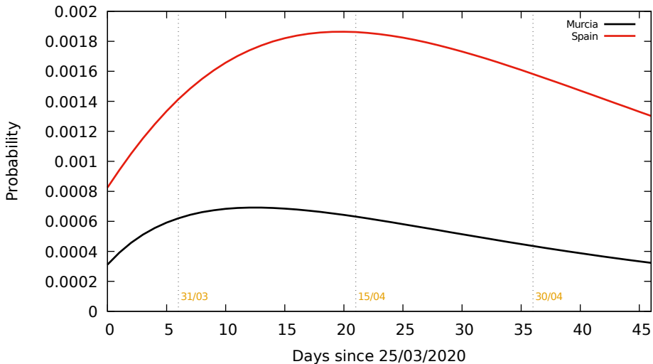
Probability of infection from detected cases only
